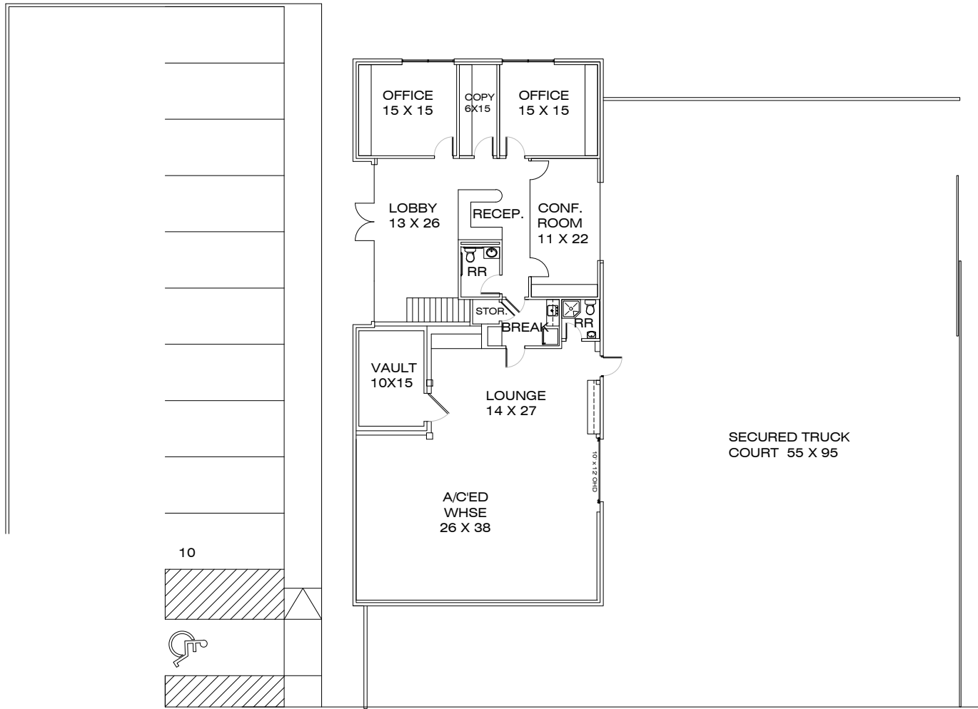
1 EXISTING FLOOR PLAN SCALE: NTS 1ST FLR OFFICE SF: 3,423
