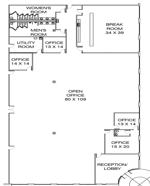
NORTH OFFICE FLOOR PLAN
