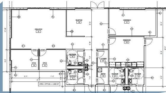
ENLARGED SPEC OFFICE PLAN
